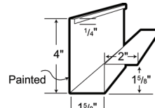
LG 133 TOP MOUNT TRACK COVER
