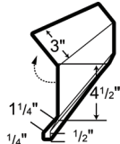
LG 119 EAVE FLASHING
