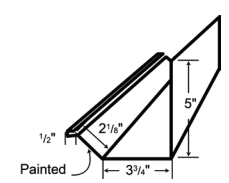
LG 148 "F" CHANNEL
