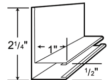
LG 148 "F" CHANNEL
