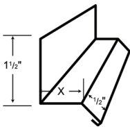
LG 129 WINDOW DRIP CAP*
